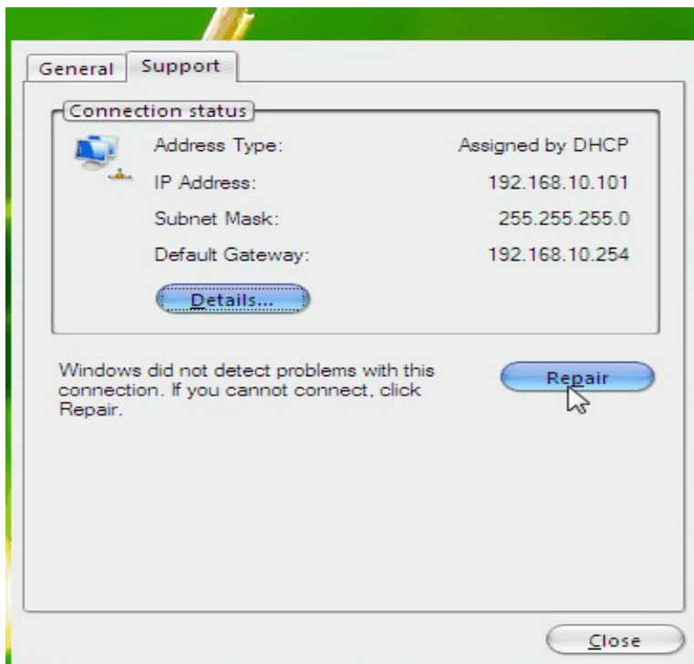
Gambar 9.3 Tampilan Repair
